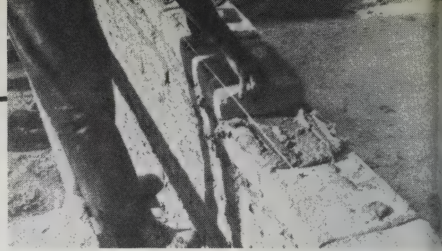
Adobe bricks being laid up in the wall. Ends and corners of wall (leads) are measured and leveled carefully, with bricks in between laid to the string stretched between leads.
